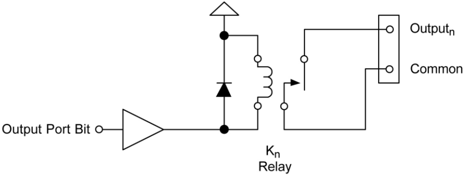
Output Circuit
