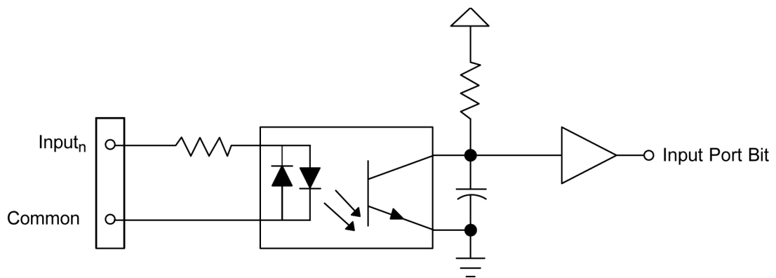
Input Circuit
