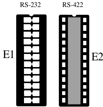
Figure 8 - Headers E1 & E2, RS-232 Selected
