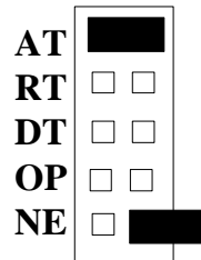
Figure 3 - Header E4, RS-485 'Auto' Enabled, with 'Echo'
