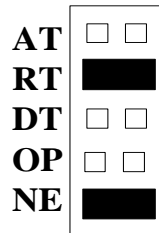
Figure 4 - Header E4, RS-485 'RTS' Enabled, with 'No Echo'
