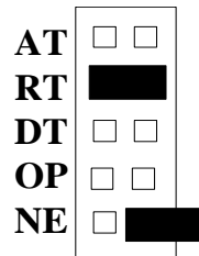
Figure 5 – Header E4, RS-485 'RTS' Enabled, with 'Echo'
