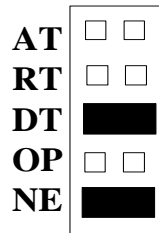
Figure 6 – Header E4, RS-485 'DTR' Enabled, with No Echo
