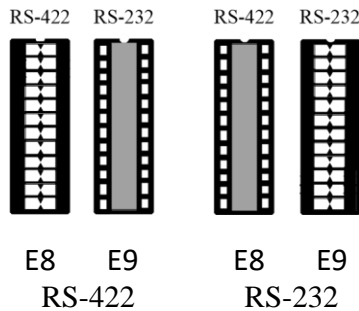
Figure 3 Headers E8 & E9, Electrical Interface Selection
